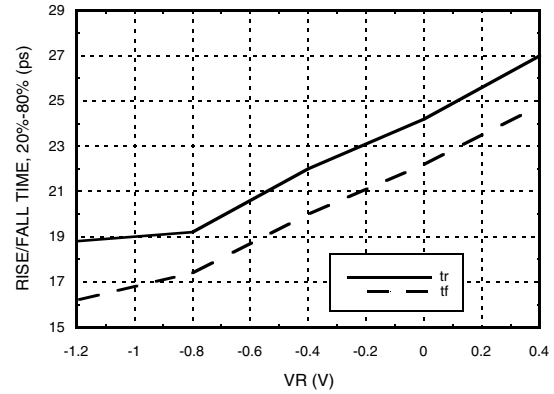
Rise / Fall Time vs. VR [3][4]
