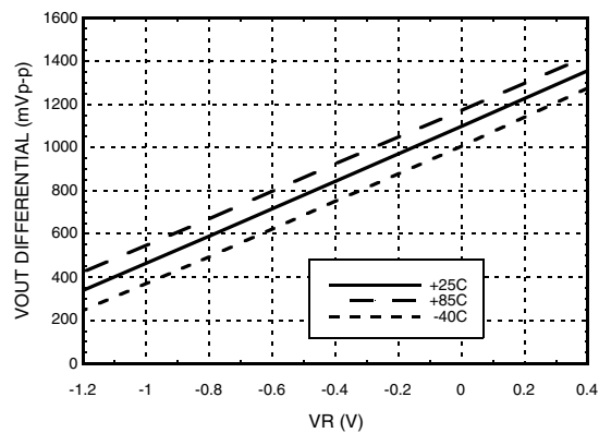
Output Differential Voltage vs. VR [2][4]
